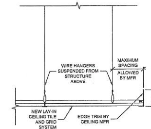
C "Cloud" Edge Detail A1.3 3/32" = 1'-0"
