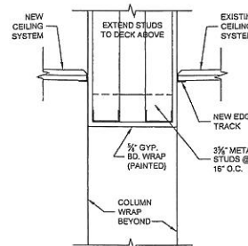
D Bulkhead Detail A1.3 3/32" = 1'-0"
